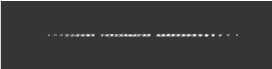
Figure 7.15. Image of fluorescence from about 40 trapped mercury ( ^{199}\text{Hg}^+ ) atomic ions. The ions are spaced by approximately 15 micrometers, and the two apparent gaps are different isotopes of mercury which do not respond to the probe laser. Reprinted courtesy of D. Wineland, at NIST.
